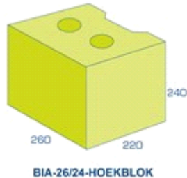
BIA-26/24-HOEKBLOK
