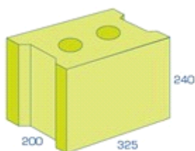
BIA-20/24
